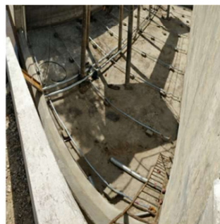
UV system installed at Sanjauli
